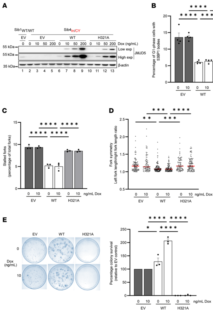
Figure 6. Decreased replication fidelity and viability of affected patient cells are due to loss of JMJD5 hydroxylase activity. Reconstitution of Sib4 in/CY fibroblasts with JMJD5. Sib4 in/CY cells were transduced with lentivirus encoding doxycycline-inducible WT or inactive (H321A) JMJD5 cDNA or a control empty vector (EV). Sib1 WT/WT cells were transduced with EV as a control. (A) Cells were treated with doxycycline for 14 days before Western blotting and immunofluorescence (Supplemental Figure 22A). “Low” and “High” refer to the exposure time. Note the leaky physiological re-expression of exogenous JMJD5 in the absence of doxycycline. (B–E) Because of modest heterogeneity in re-expression levels between cells (Supplemental Figure 22A), and slightly reduced expression of H321A compared with WT JMJD5, all subsequent experiments were conducted at 0 and 10 ng/mL doxycycline. Increased 53BP1 bodies (B), stalled replication forks (C), and replication fork asymmetry (D) in Sib4 in/CY cells are suppressed by JMJD5 hydroxylase activity. (E) Decreased colony survival of Sib4 in/CY cells is rescued by JMJD5 hydroxylase activity. Reconstituted Sib4 in/CY cells were plated at limited density and monitored for colony formation. Left: Example of stained colonies. Right: Quantification of colonies expressed as percentage survival relative to Sib4 in/CY EV control cells. In B, a minimum of 300 cells were counted per condition. In C, at least 200 forks were counted per sample. In D, at least 50 structures per condition were measured in each experiment. (B) Data represent mean ± SEM from 4 independent experiments. (C–E) Data represent mean ± SEM from 3 independent experiments. Statistical analyses used 1-way ANOVA with Tukey’s post hoc test (B, C, and E) or Kruskal-Wallis with Dunn’s correction (D); *P ≤ 0.05, **P ≤ 0.01, ***P ≤ 0.001, ****P ≤ 0.0001.
